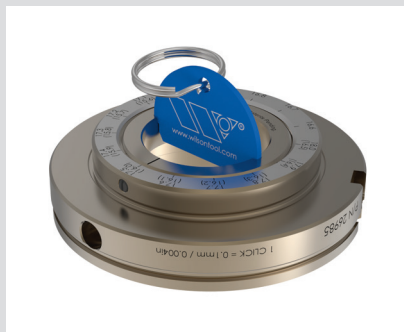
Step 2. Adjust shimless adapter
