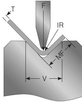
Required Press Force for 90° Air Bends
