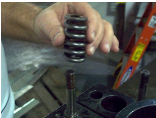
10. Take the spring off the punch.
