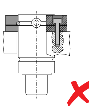
Installation NOT allowed due to tensile stress on screws.
