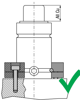
Installation with bracket mount flange.
