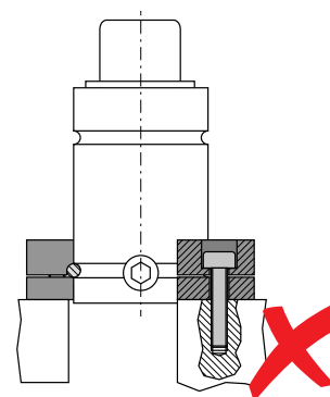
Installation NOT allowed due to excessive stress on gas spring body and flange.
