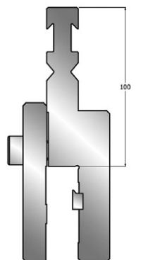
Adaptor RFA-RFA
