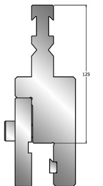
Adaptor RFA-R
