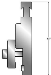
Adaptor R-EuroA
