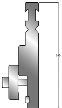
Adaptor RFA-EuroA
