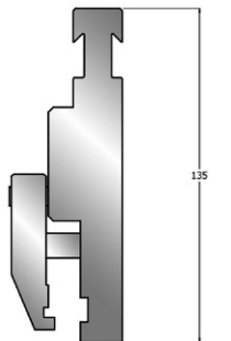
Adaptor R-EuroB
