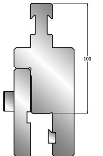
Adaptor R-R
