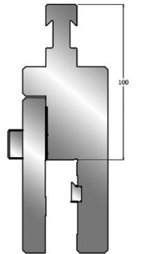
Adaptor R-RFA
